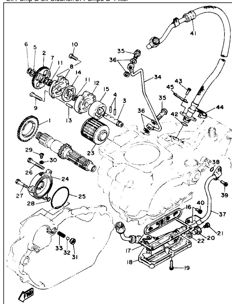
Baugruppe Oil Pump & Oil Cleaner/Öl-Pumpe & -Filter Figure/Bild 6
