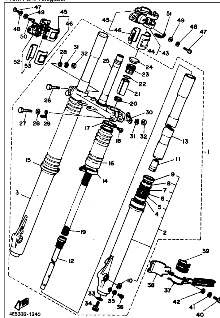
Front Fork/Telegabel
